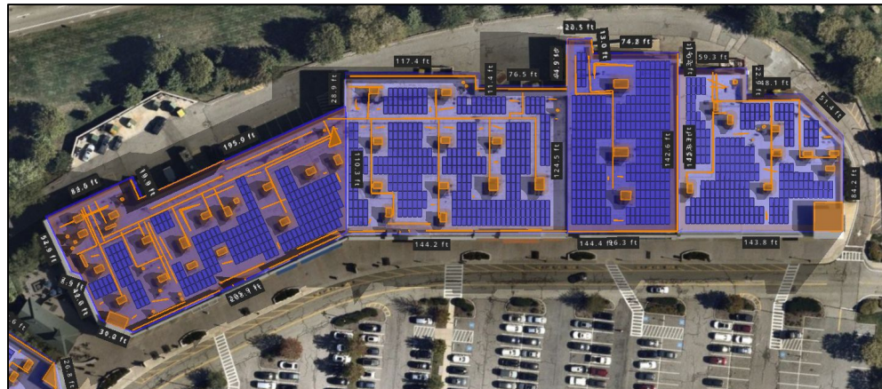
Sample solar layout in Helioscope CAD software.
